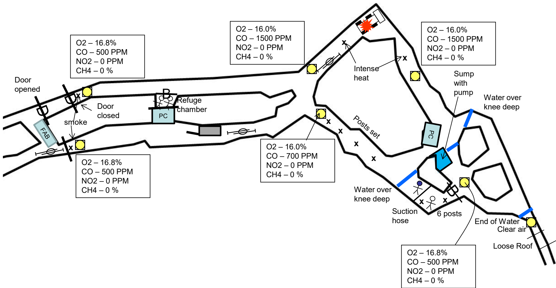
Mine 1 Problem Map
