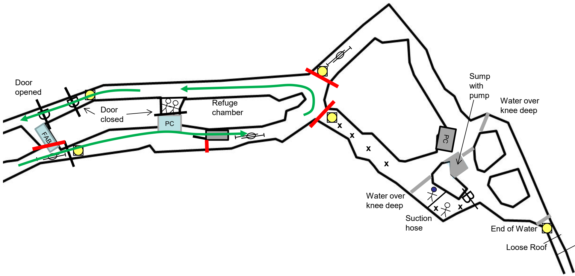
Mine 1 1 st Ventilation
