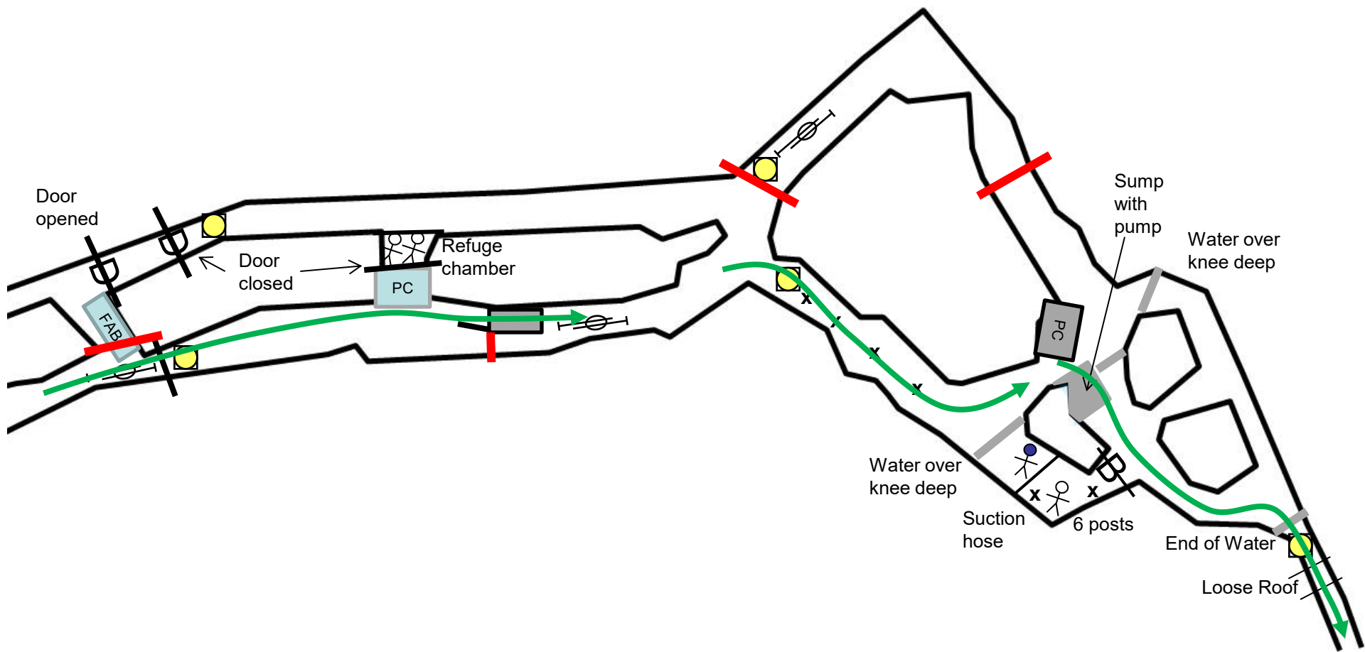
Mine 1 2nd Ventilation
